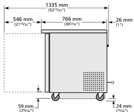
RIGHT VIEW
